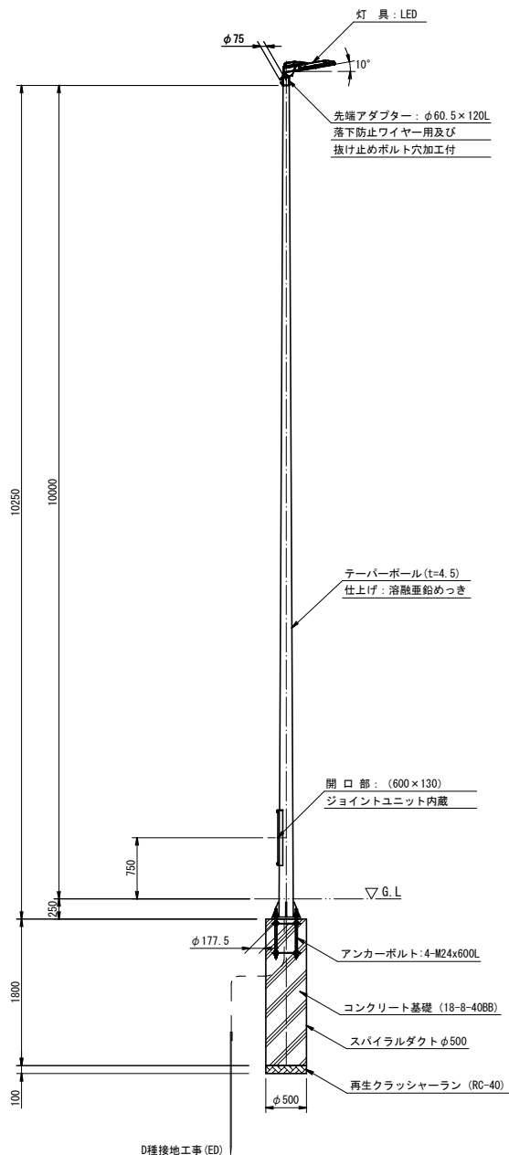
照明柱姿図 1: 30 (A1) 1: 60 (A3)
